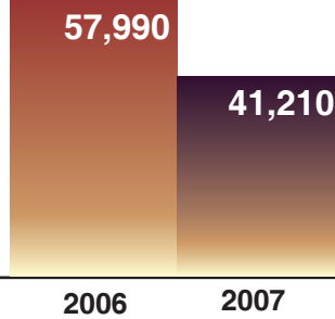
Website Hits
