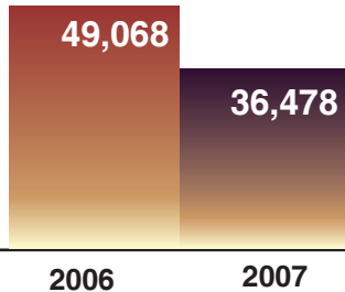
Database Searches
