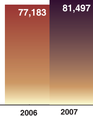
Internet Sign-Ins
